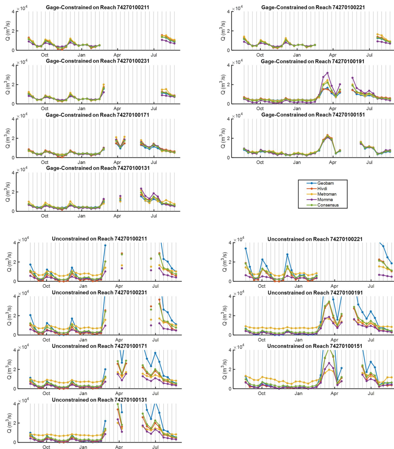
Figure 7. Example simulated Surface Water and Ocean Topography (SWOT) discharge ( Q ) results mimicking Agency-led data products for seven reaches on the Mississippi River. Branch (i.e., either gage-constrained or unconstrained) and SWOT mission river database (SWORD) reach IDs are shown in titles of each subplot. The various colored lines indicate each flow law parameter estimation algorithm, and are labeled in the figure legend. Note that some values exceed Y axis limit.
